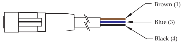
Figure 4.7: Analog output cable signal information
