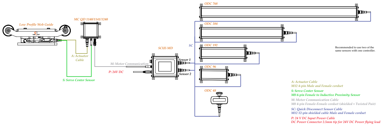
Figure 6.2: Wiring example with a displacement guide.
