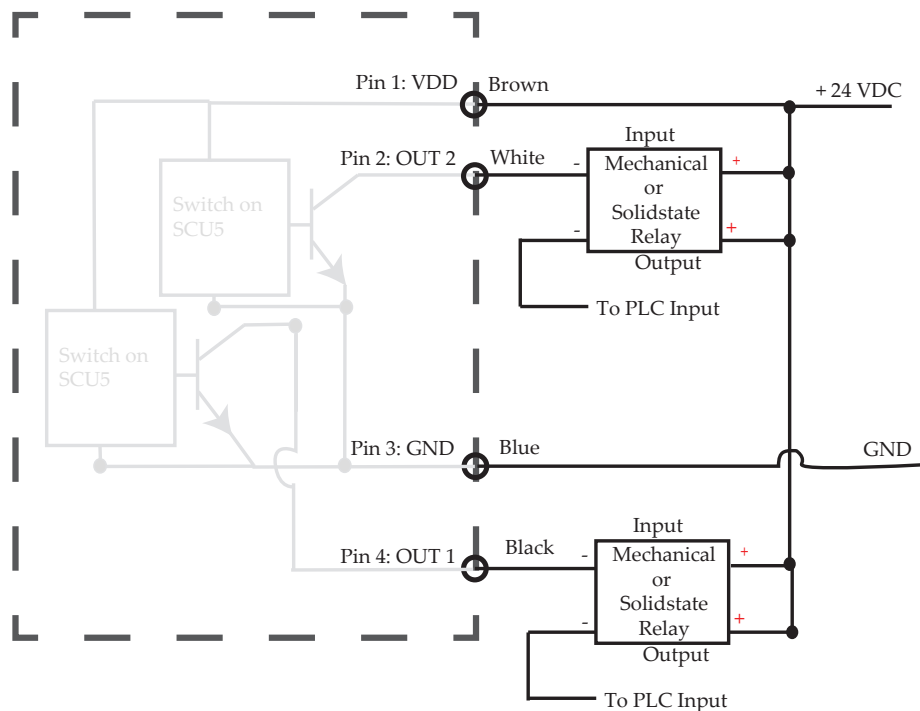
Figure 4.11: Typical wiring information for NPN normally closed output from SCU5 Controller to PNP inputs in a PLC
