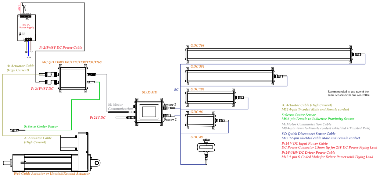
Figure 6.3: Wiring example with a unwind/rewind actuator.
