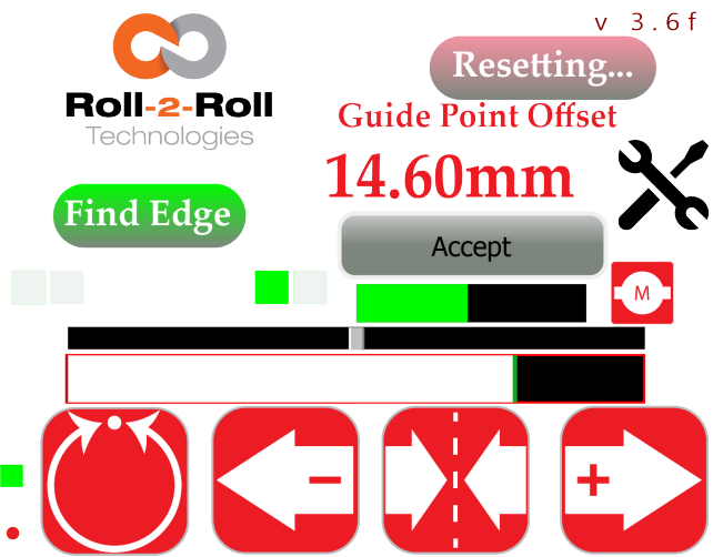
Figure 5.33: Temporary guide point change based on the current web position is displayed
