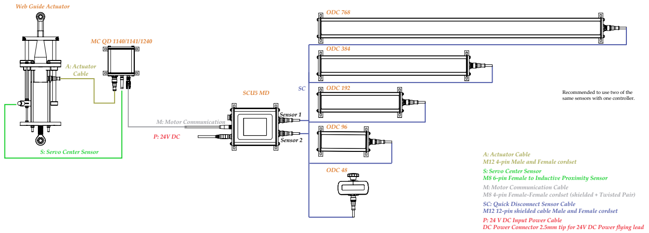
Figure 6.4: Wiring example with web guide upgrade actuator.
