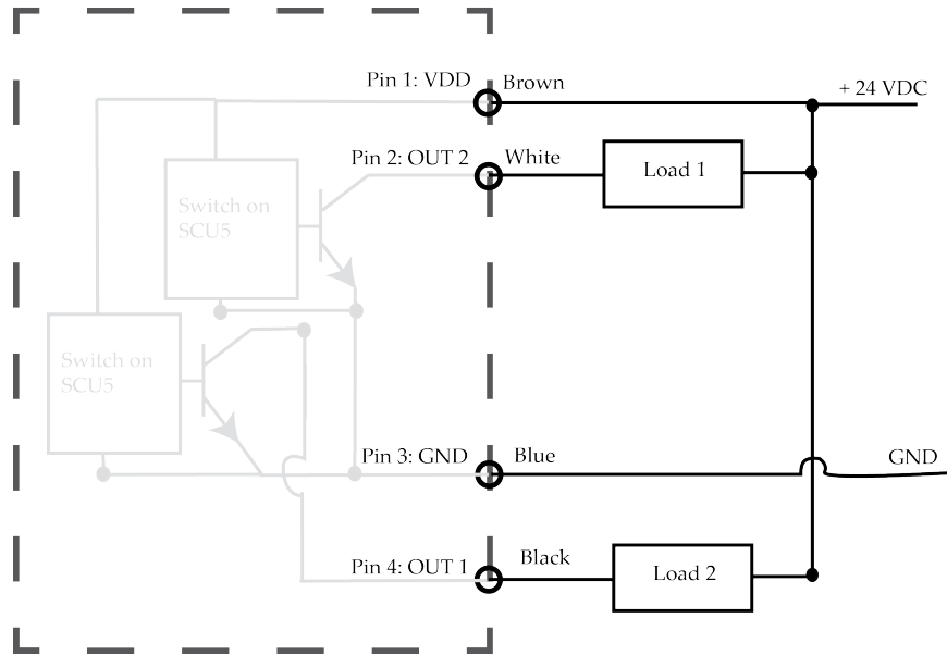
Figure 4.10: Typical wiring information for NPN normally closed output from SCU5 Controller
