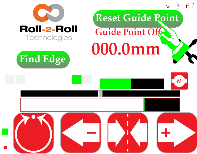
Figure 5.32: Guide point reset initiated by pressing reset guide point button
