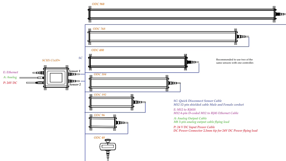
Figure 6.1: Wiring of the SCU5 controller for sensing and measurement applications.
