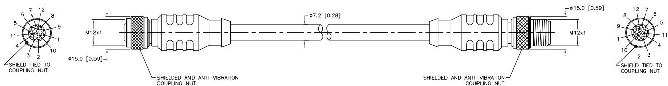
Figure 4.4: Quick Disconnect Sensor Cable
