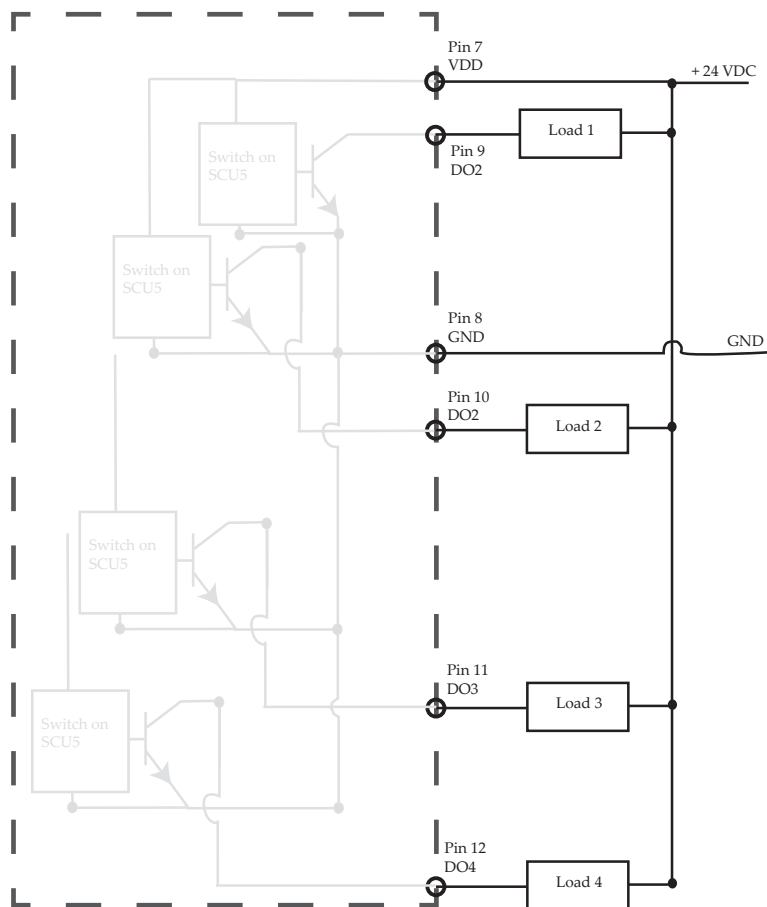
Figure 4.14: Typical wiring information for NPN normally closed output from SCU5 controller
