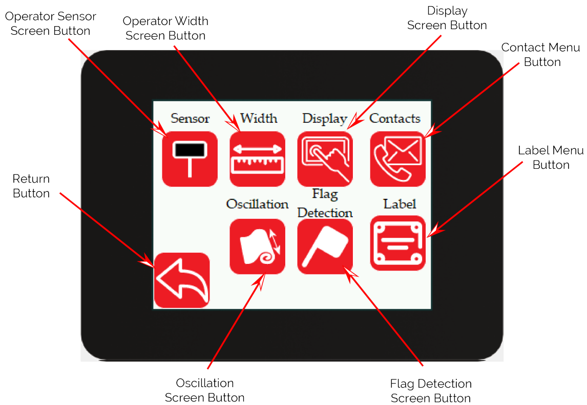
Figure 5.54: Operator Menu Screen
