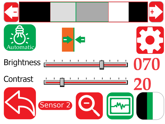
Figure 5.60: Edge created by two colors (Teaching Saved)
