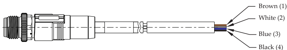
Figure 4.9: M12 4-pin digital IO cable information
