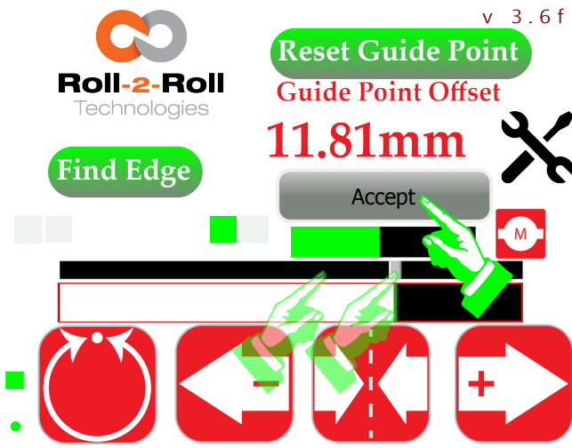
Figure 5.30: Gross guide point change needs to be accepted
