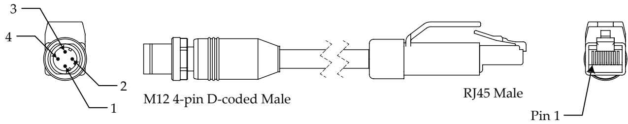
Figure 4.8: M12 to RJ45 cable information
