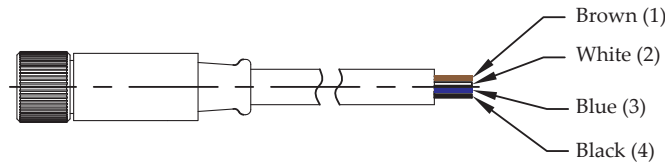
Figure 4.6: Digital input cable signal information
