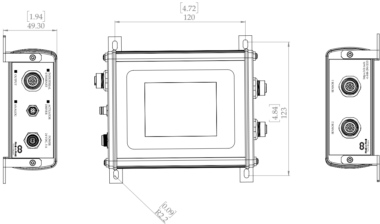
Figure 4.1: SCU5 controller Physical Dimensions (All dimensions are in mm [in]); Subject to change without notice.
