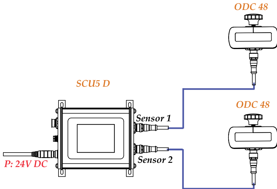
Figure 3.1: SCU5 Controller with two Roll-2-Roll® Sensors
