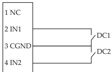
Figure 4.12: Typical wiring information for dry contact inputs
